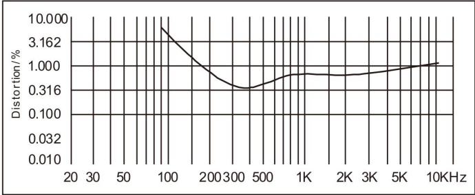
Distortion (THD<1.5% 1W, 1m,200Hz-10kHz)
