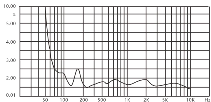
DSP8063 Distortion
